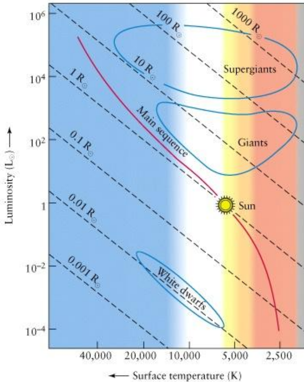
Sizes of stars in different locations on the H-R diagram
